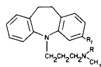
Scheme I
